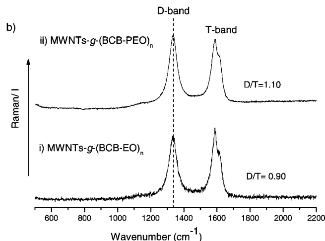
Figure 6. (a) FT-IR of MWNTs- g -(BCB-PEO) n recovered from the reaction carried out for 4 h in THF at 50 °C and b) Raman spectra of precursor initiator (3) and surface-initiated PEO (5) attached MWNTs, (i) MWNTs- g -(BCB-EO) n and (ii) MWNTs- g -(BCB-PEO) n .
