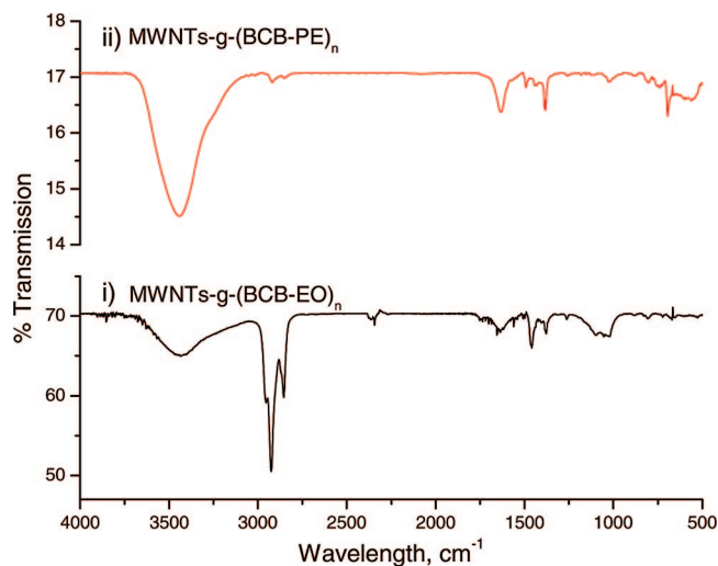
Figure 3. FT-IR spectra of precursor initiator functionalized MWNTs. (i) MWNT- g -(BCB-EO) n and (ii) MWNTs- g -(BCB-PE) n (Table 1, runs 1 and 4).
